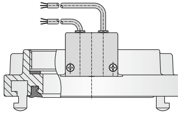
Fixed coupling
